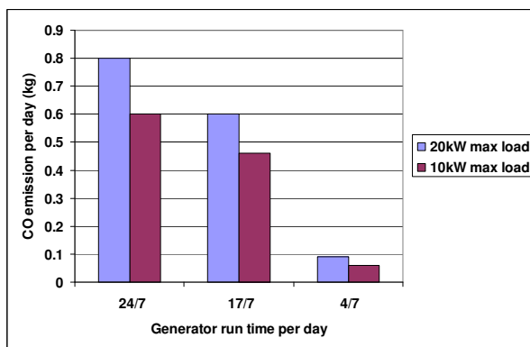
Graph 30 Similarly, CO emission is also reduced by a higher factor than diesel consumption.
