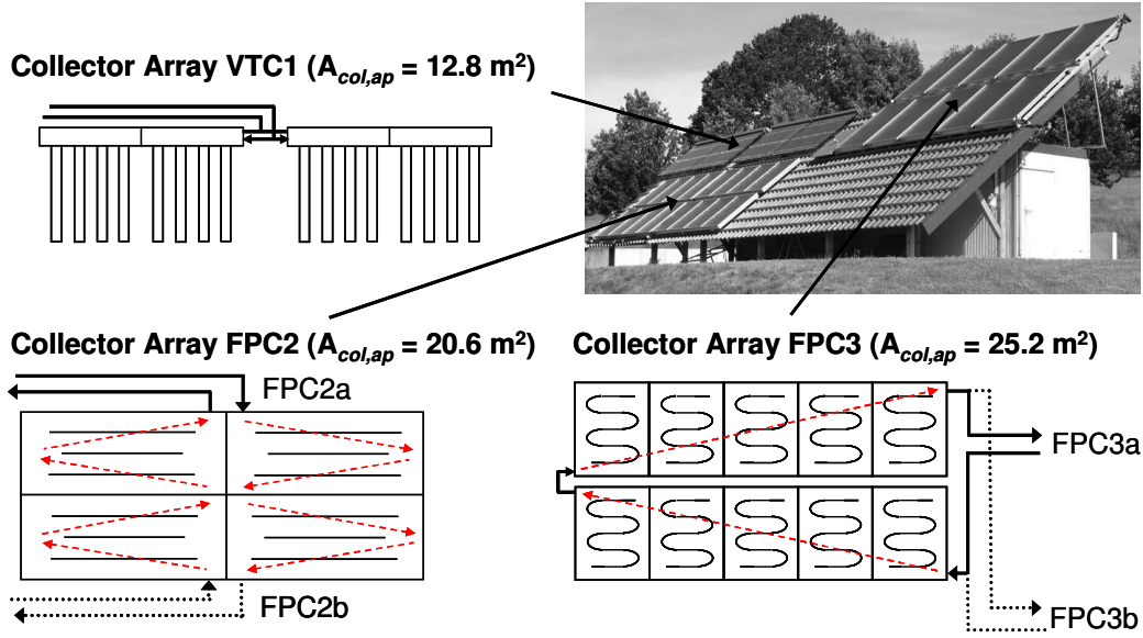
Fig. 1. Schematic sketch of the three investigated collector array hydraulics. At the flat-plate collectors experiments with unfavourable (FPCxa) and optimized external piping (FPCxb) were carried out.
