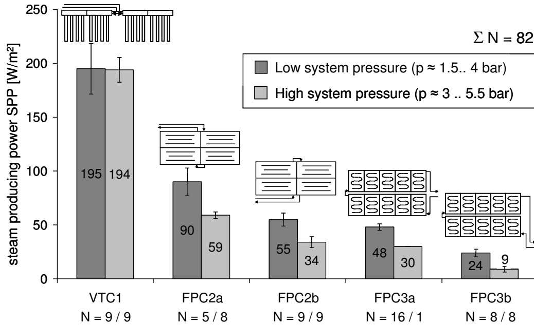
Fig. 2. Measured mean steam producing power (SPP) for different collector loop gage pressures and different external collector array piping. The values of system pressure refer to the static and maximum pressure. N termed the number of experiments for each bar. The error bar marks the standard deviation of the measured mean SPP.
