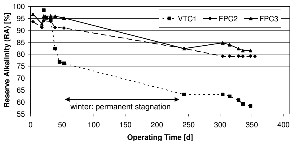
Fig. 3. Reserve alkalinity (RA) as a function of operating time of the three investigated test systems. Replenishment of new solar fluid leads to temporary increase of RA. Day 0 was 01.08.2004.
